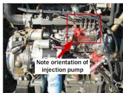
YANMAR TK482 OR TK486 (from 1998 to 2002+)
